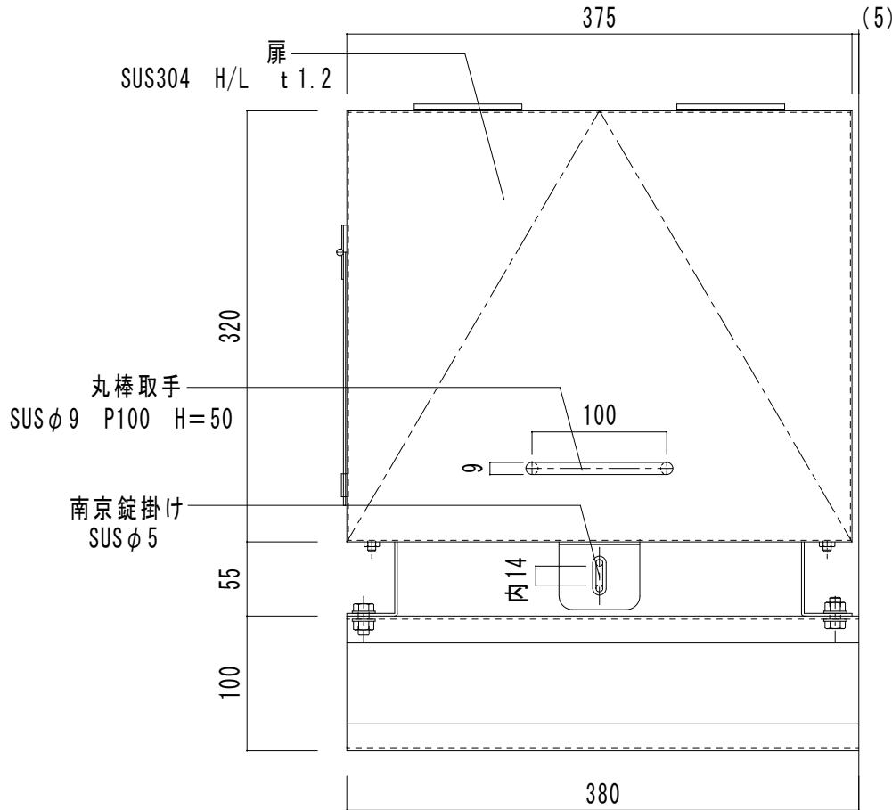
矢視; A (S=1/5)
